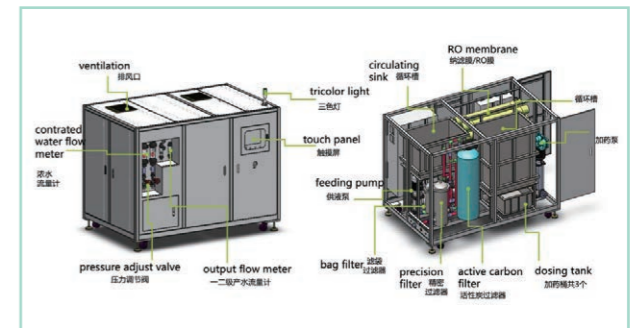
On-line Water Recovery System
